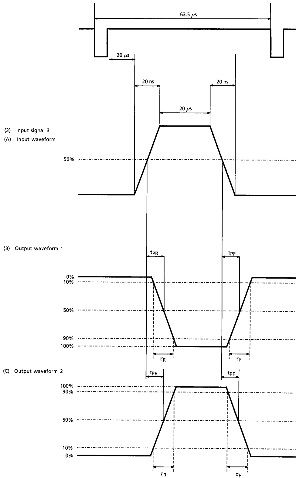
Fig.T-2 Test pulses for TA1310BN test stage
