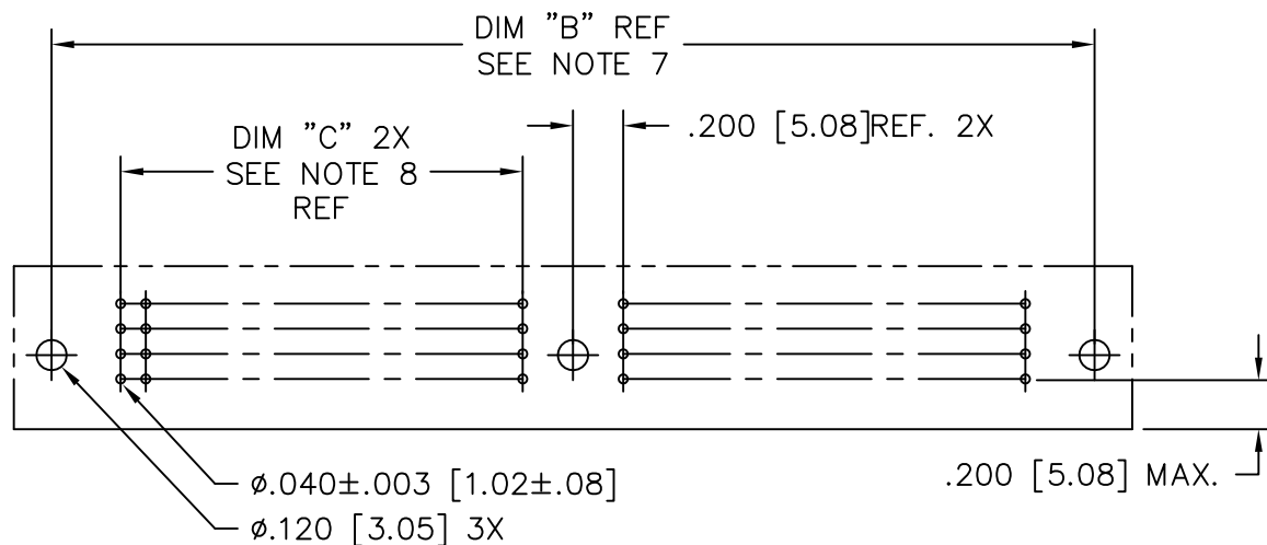
SECTION U-U
