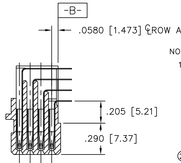
SECTION X-X
