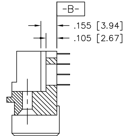
SECTION W-W
