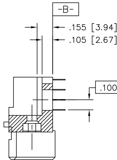
SECTION U-U
