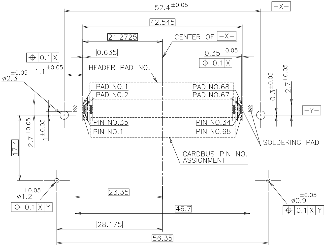
PCB LAYOUT VIEW B SCALE:2:1 コネクタ搭載部詳細 CONNECTOR MOUNTING LAYOUT
