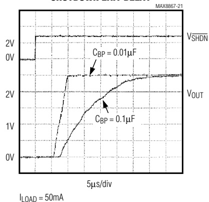
MAX886_EUK25 SHUTDOWN EXIT DELAY
