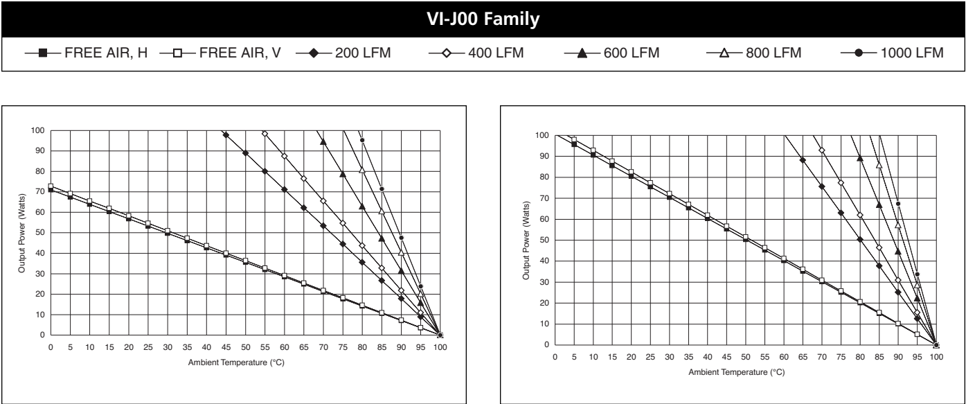
Figure 21-17 — VI-J00 Family, Part #30140 heat sink 5 V output
