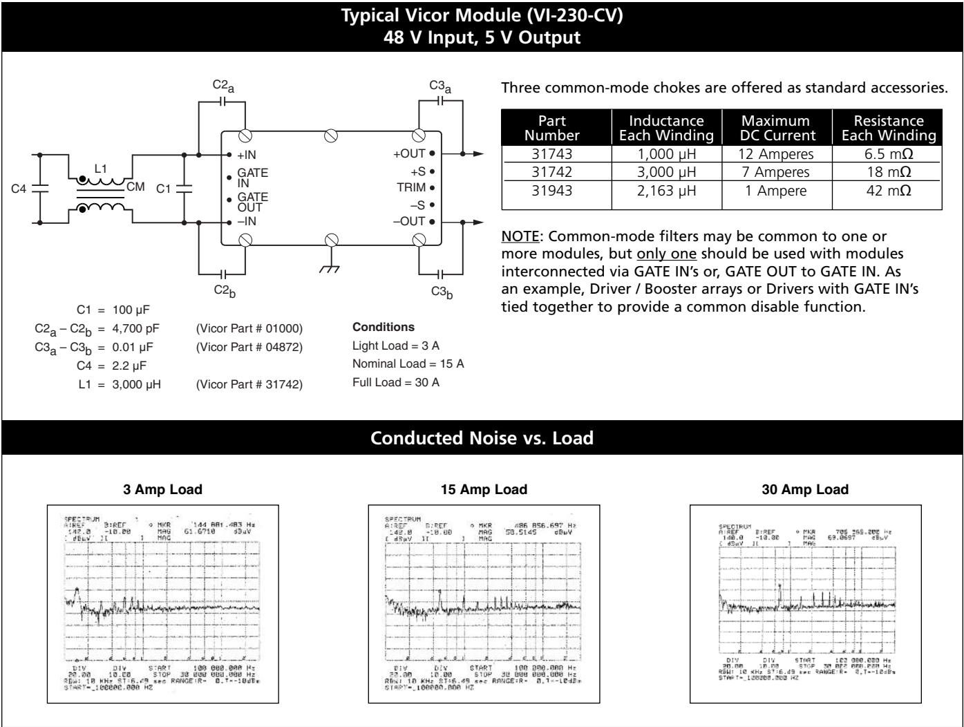
Figure 9-3 — Conducted input noise, with common-mode choke
