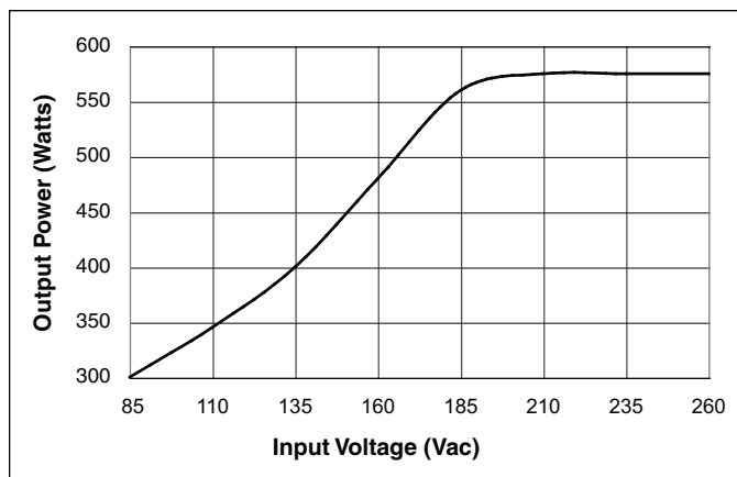
Figure 19-5 — Output power start-up de-rating @ -30^{\circ}\text{C} (I-Grade only). 5 minute warm up required before full power (see Figure 19-1) is available.
