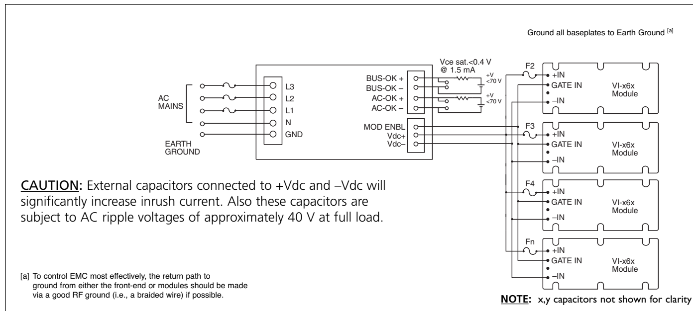
Figure 16-3 — 1.5, 3.0 kW Front-end
