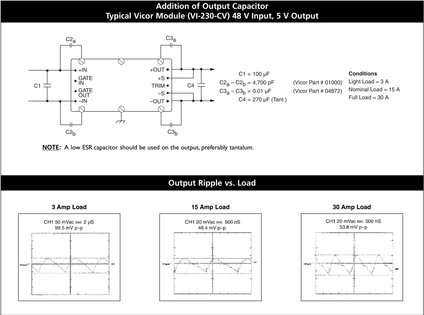
Figure 9-11 — Output noise, additional output capacitance
