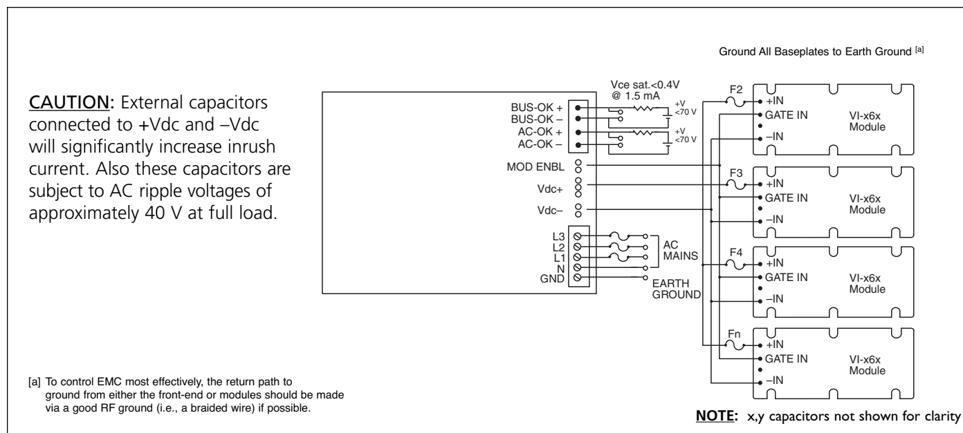
Figure 16-4 — 5.0 kW Front-end
