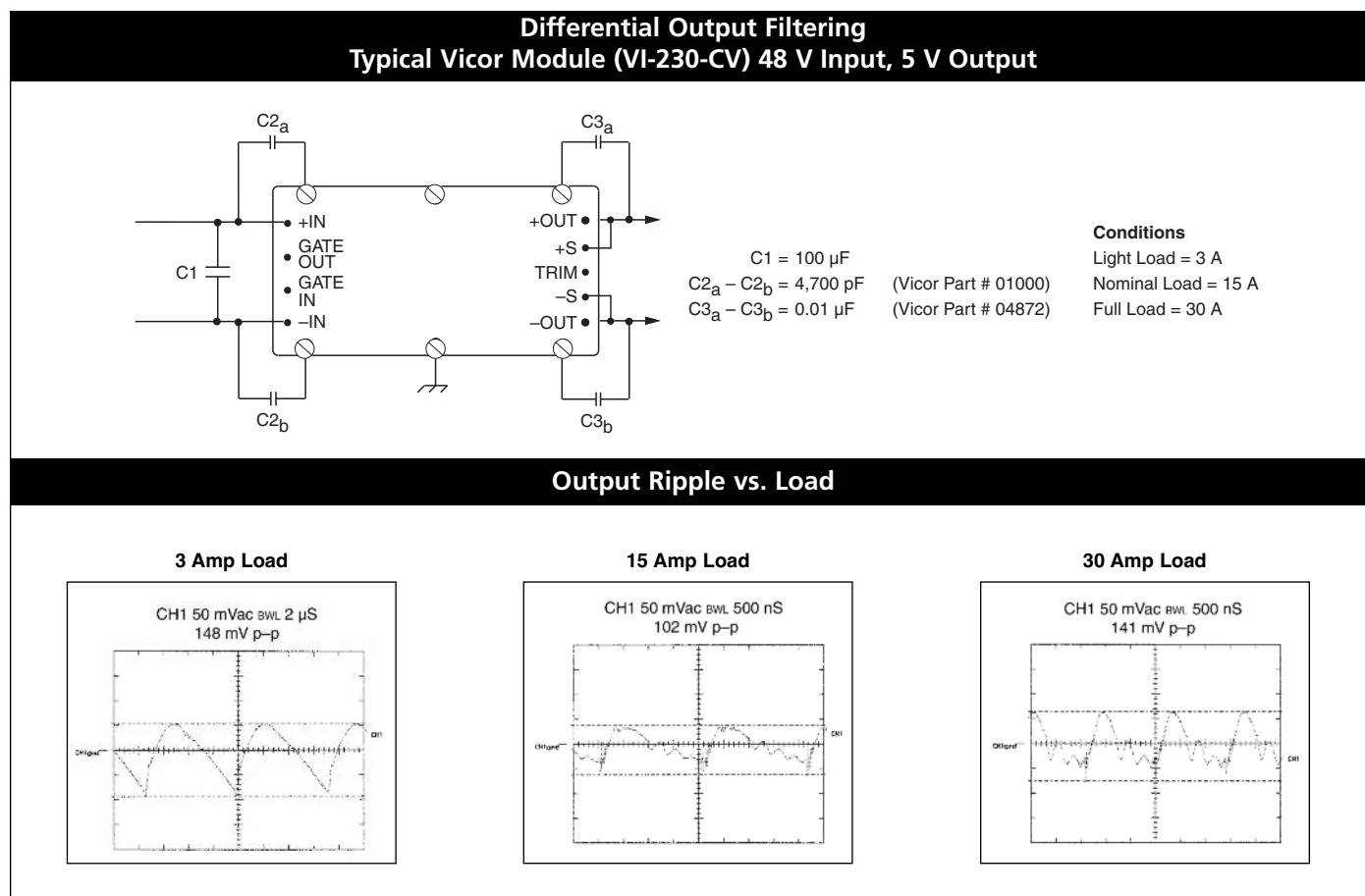
Figure 9–10 — Output noise, no additional output filtering
