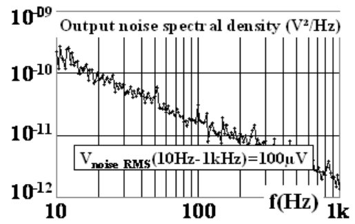
Figure 8: S_{V_{\text{out}}}(\text{V}^2/\text{Hz}) @ 25^{\circ}\text{C} , I_{\text{Load}}=100\text{mA}
