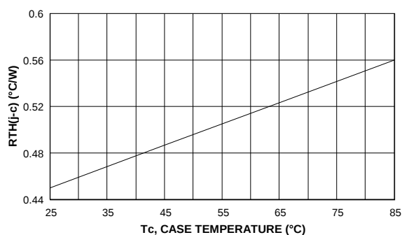
Figure 8. Maximum thermal resistance vs case temperature
