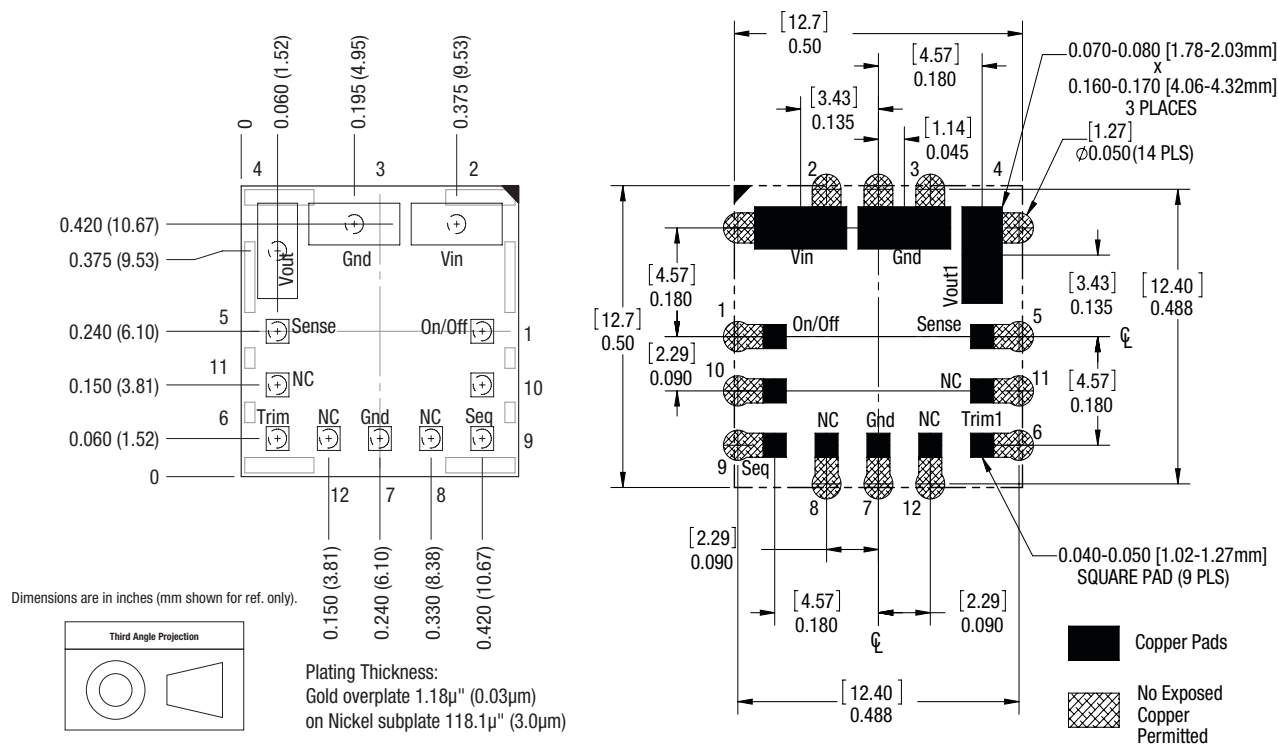
Figure 3. OKL-T/6-W5 Mechanical Outline
