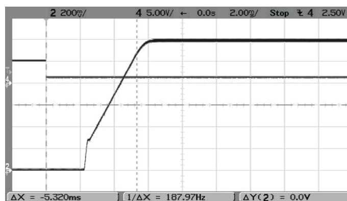
On/Off Enable Startup (V IN =5V, V OUT =1.2V, I OUT =6A, Load=0) Trace 4=Enable, Trace2=V OUT
