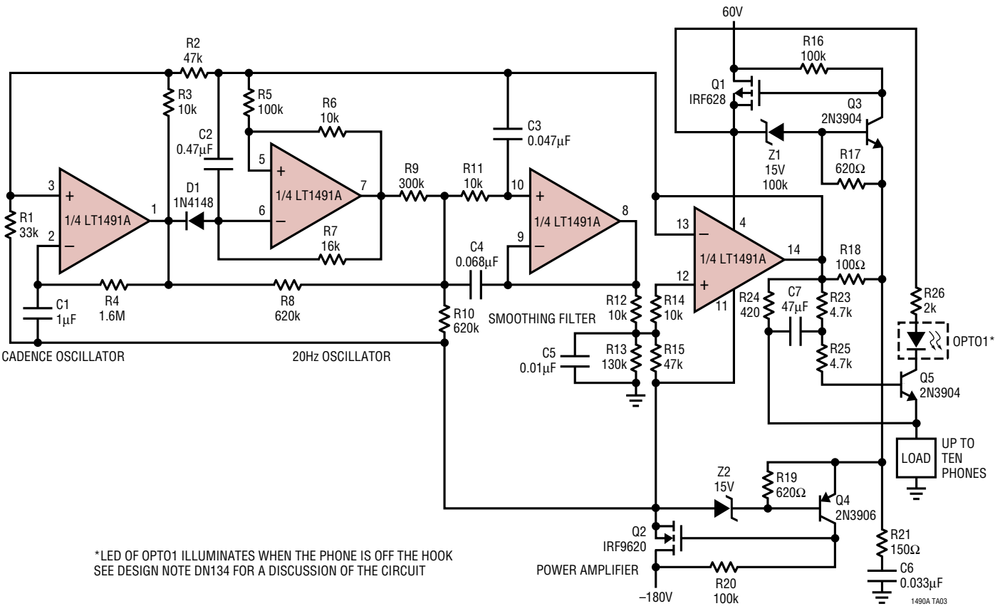
Ring-Tone Generator
