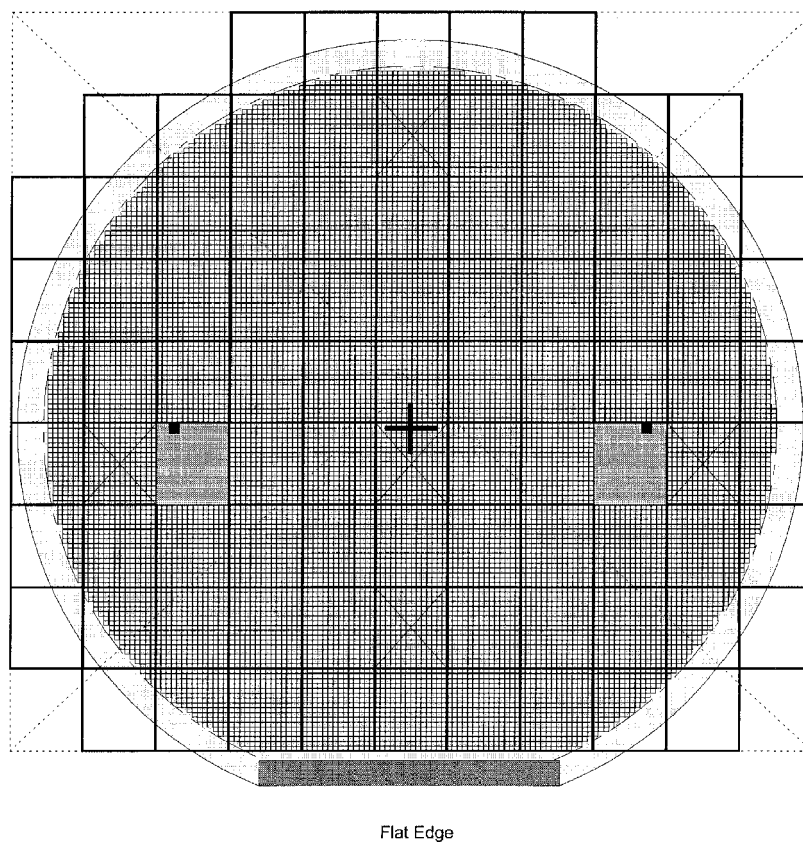
Figure 10-4. Wafer Map
