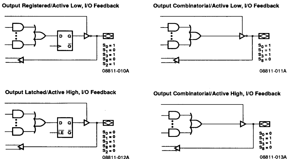
Figure 3b. Single Feedback Macrocells
