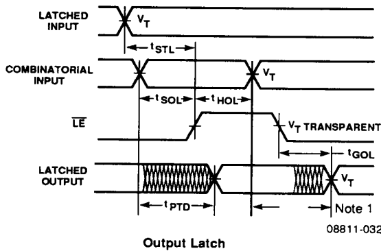
Output Latch
