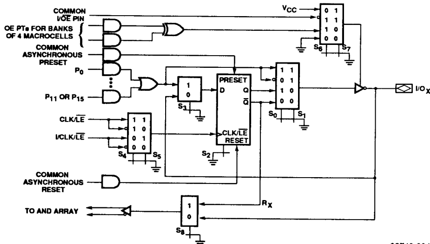
Figure 2a. PALCE29M16 Macrocell (Single Feedback)
