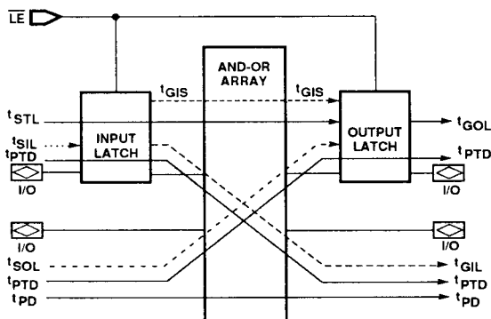
Input/Output Latch Specs
