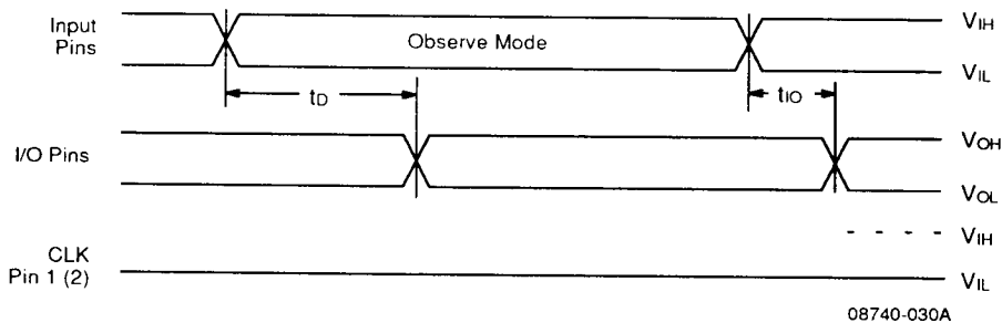
Observability Waveform
