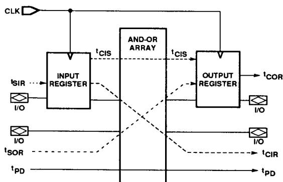
Input/Output Register Specs
