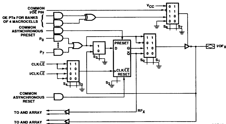
Figure 2b. PALCE29M16 Macrocell (Dual Feedback)
