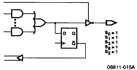
Output Combinatorial/Active Low, Latched Feedback
