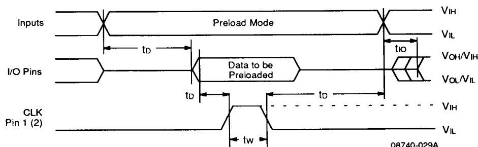
Preload Waveform
