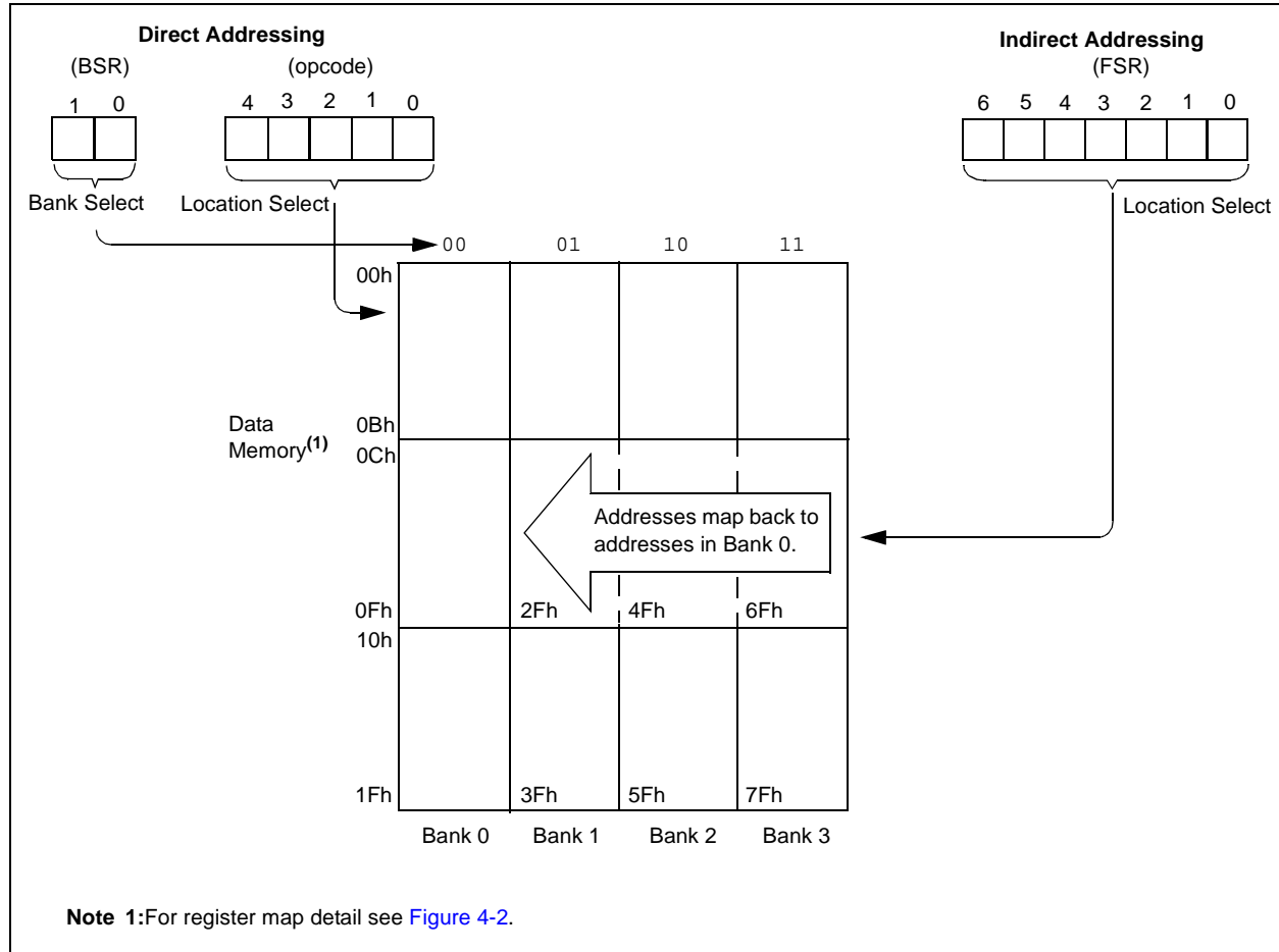
FIGURE 4-4: DIRECT/INDIRECT ADDRESSING
