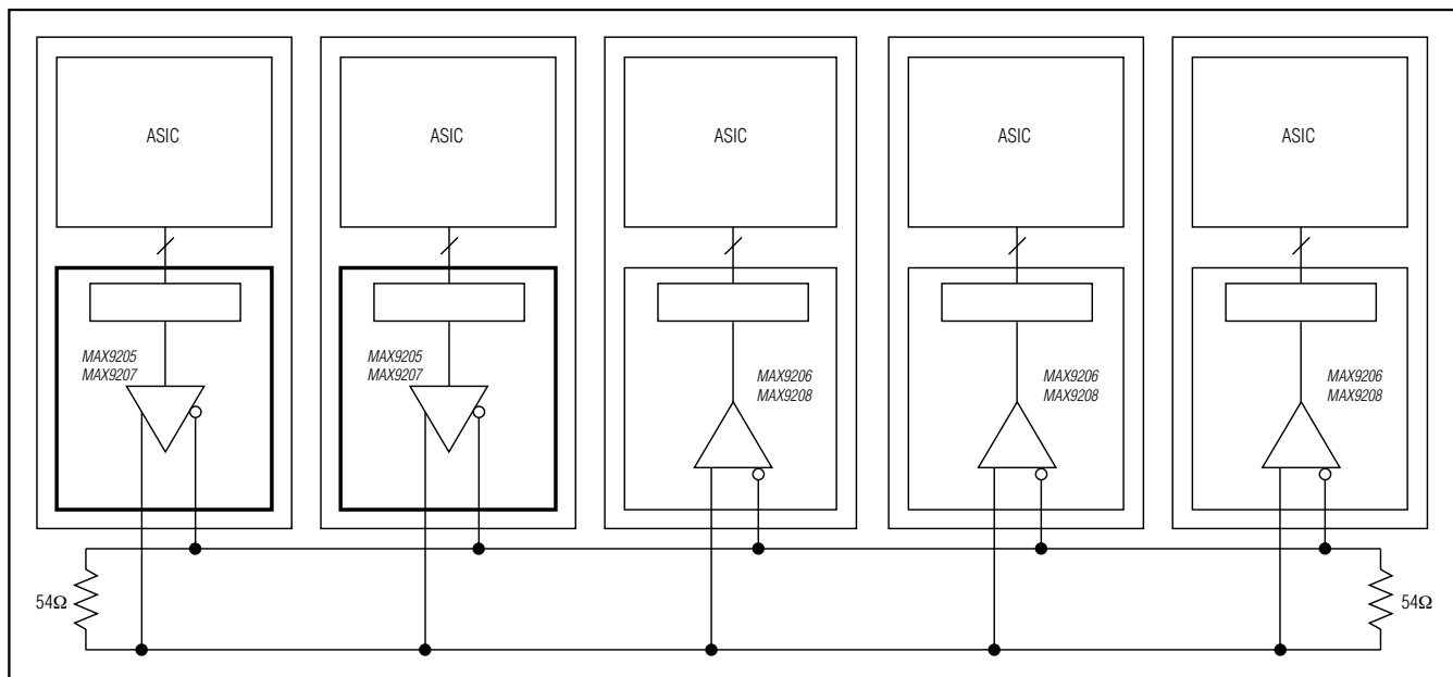
Figure 14. Multipoint
