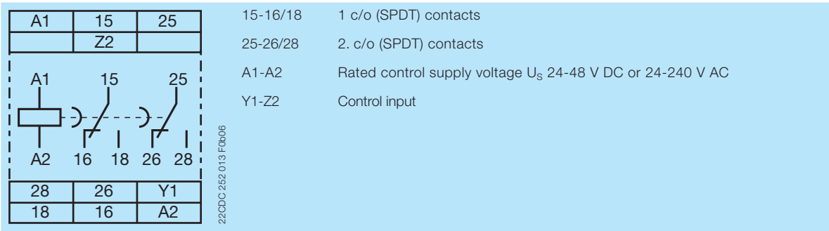
Connection diagram
