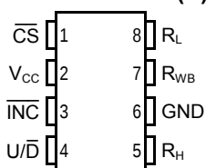
TSSOP 8-Lead (Y)
