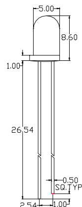
Figure 2 5mm LED
