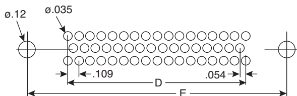
50 Pin PCB Layout
