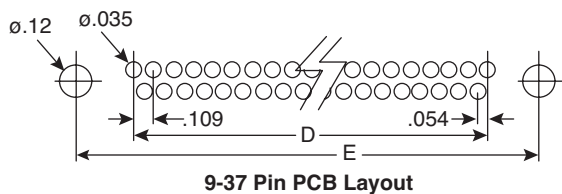
9-37 Pin PCB Layout
