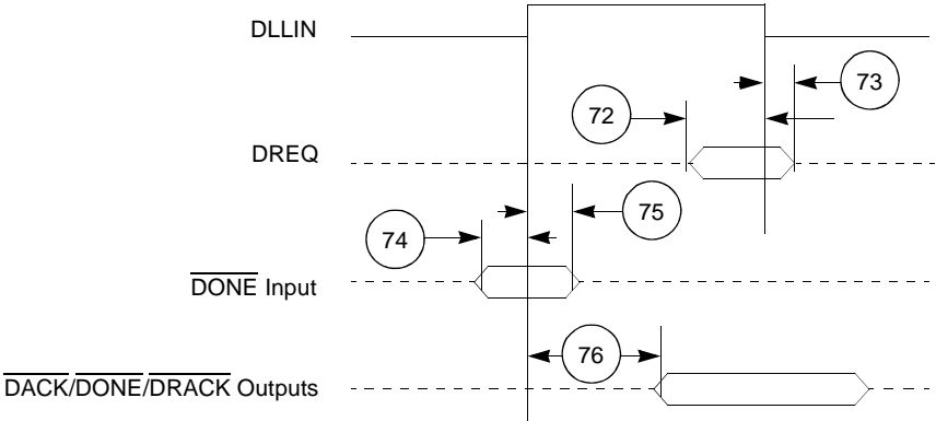
Figure 2-11. DMA Signals
