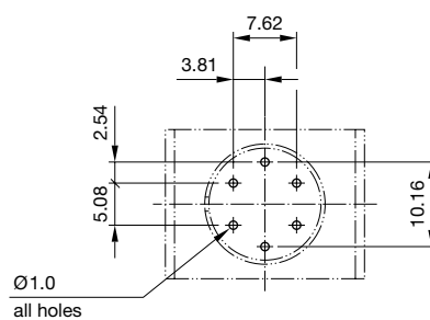
Drilling plan (solder side)
