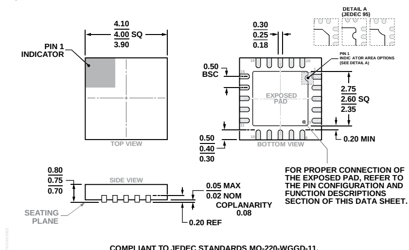
Figure 69. 20-Lead Lead Frame Chip Scale Package [LFCSP]
