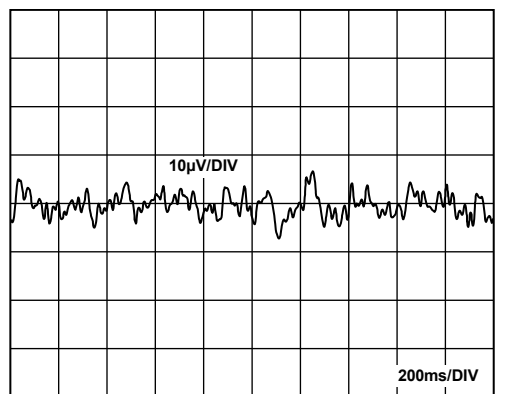
Figure 12. Instrumentation Amplifier 0.5 Hz to 40 Hz Noise
