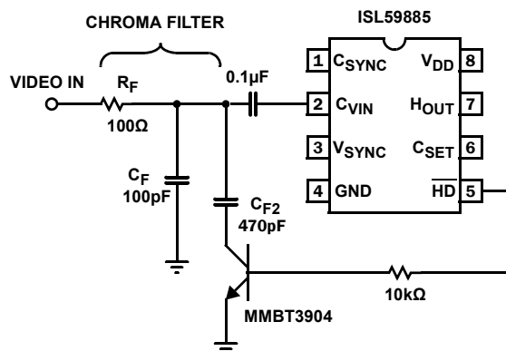
FIGURE 14. OPTIONAL CHROMA FILTER
