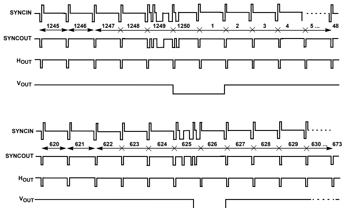
FIGURE 11. HDTV 1080i/25 LINE COMPOSITE VIDEO: INTERLACED (1250 LINES)
