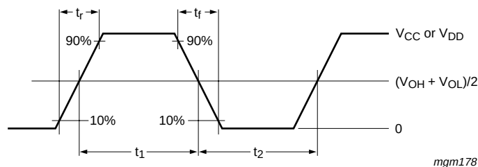
Fig 9. Definition of output transition times
