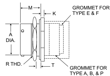
CRIMP KPSE07/MS3124
