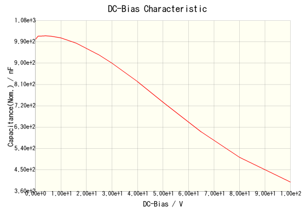
C4532X7R2A105M230KA
