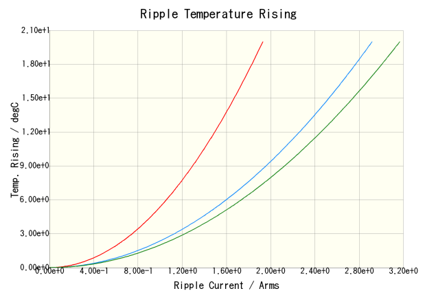
C4532X7R2A105M230KA(100kHz) C4532X7R2A105M230KA(500kHz) C4532X7R2A105M230KA(1MHz)
