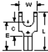
MU18-10FFB Stud Size 10 Wire Range 22-18
