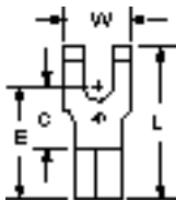
MU10-6FFB Stud Size 6 Wire Range 12-10
