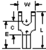
MU18-8FFB Stud Size 8 Wire Range 22-18
