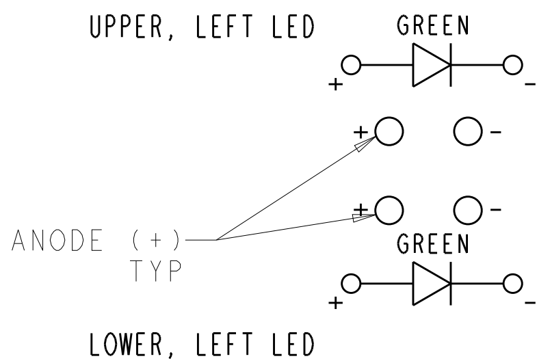
6368116-1, -2 LED SCHEMATIC
