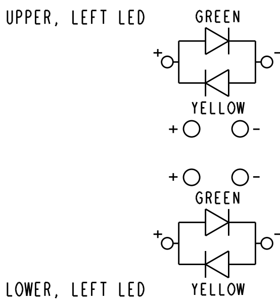
6368116-3 LED SCHEMATIC
