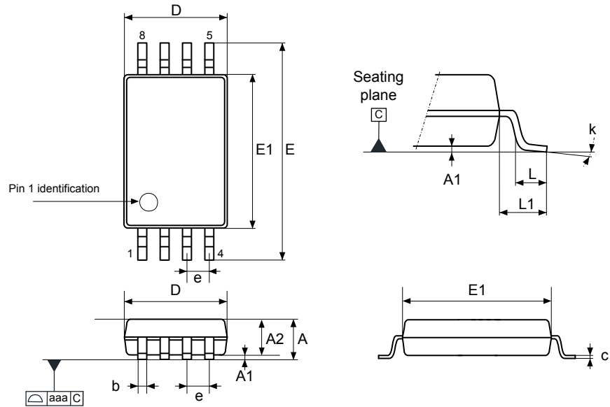
Figure 17. TSSOP8 – Outline
