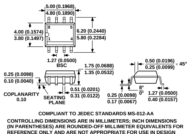
Figure 28. 8-Lead Standard Small Outline Package [SOIC_N] Narrow Body (R-8) Dimensions shown in millimeters and (inches)
