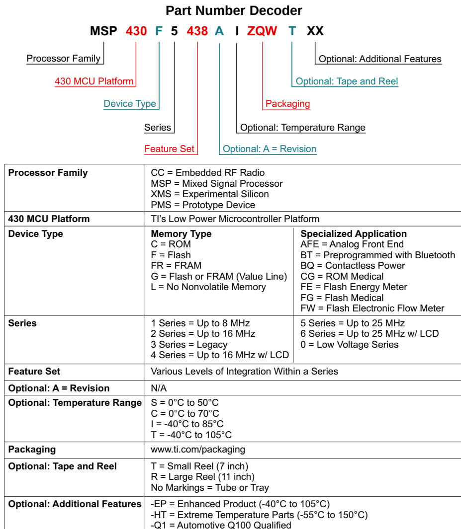
Figure 2. Device Nomenclature
