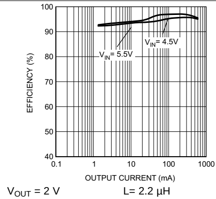
Figure 21. Efficiency vs Output Current (PWM-to-PFM Mode)
