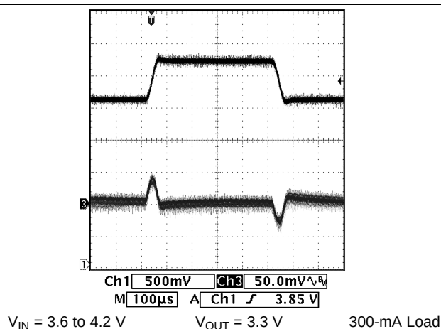
Figure 6. Line Transient (LDO2)
