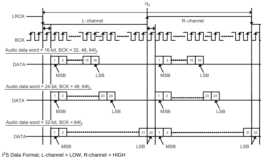
Figure 14. I²S Audio Data Format
