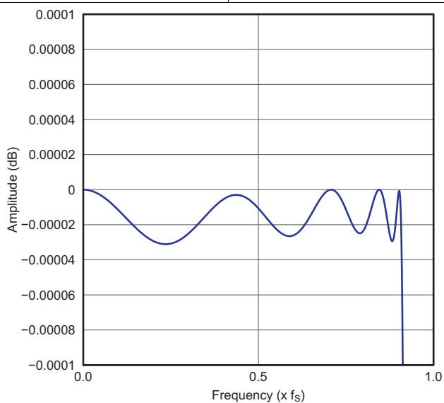
Figure 29. Low Latency x4 Interpolation Filter Passband Ripple
