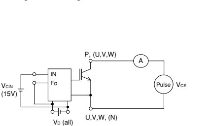
b) Upper Arm Switching
