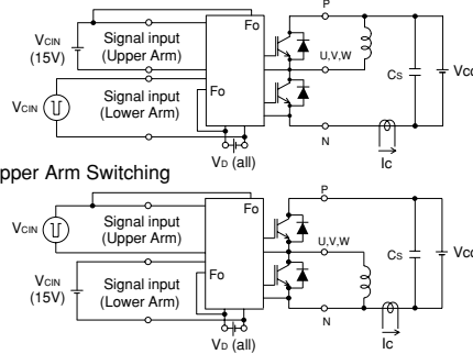
b) Upper Arm Switching
