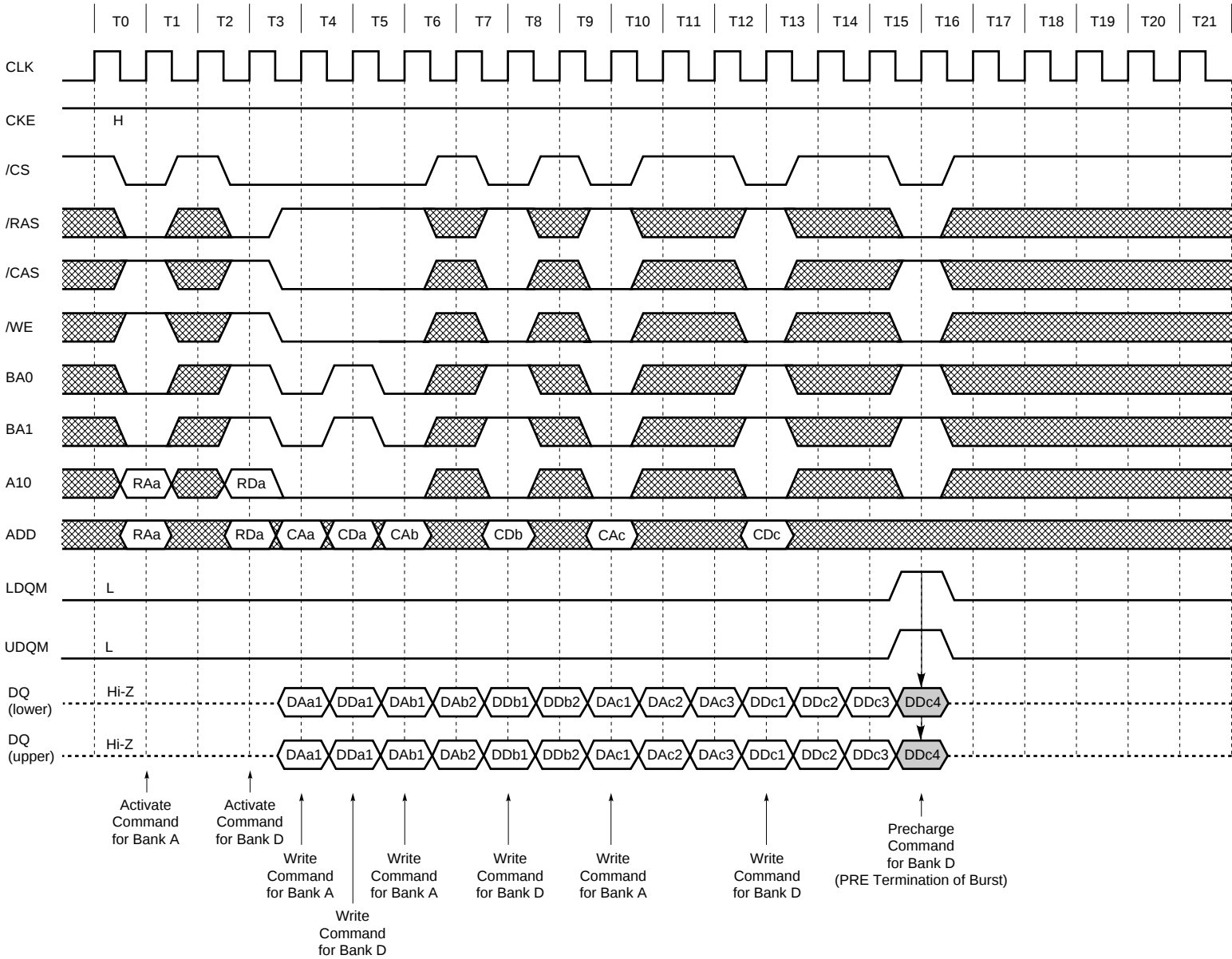
13.26 Full Page Random Column Write (Burst Length = Full Page, /CAS Latency = 2)
