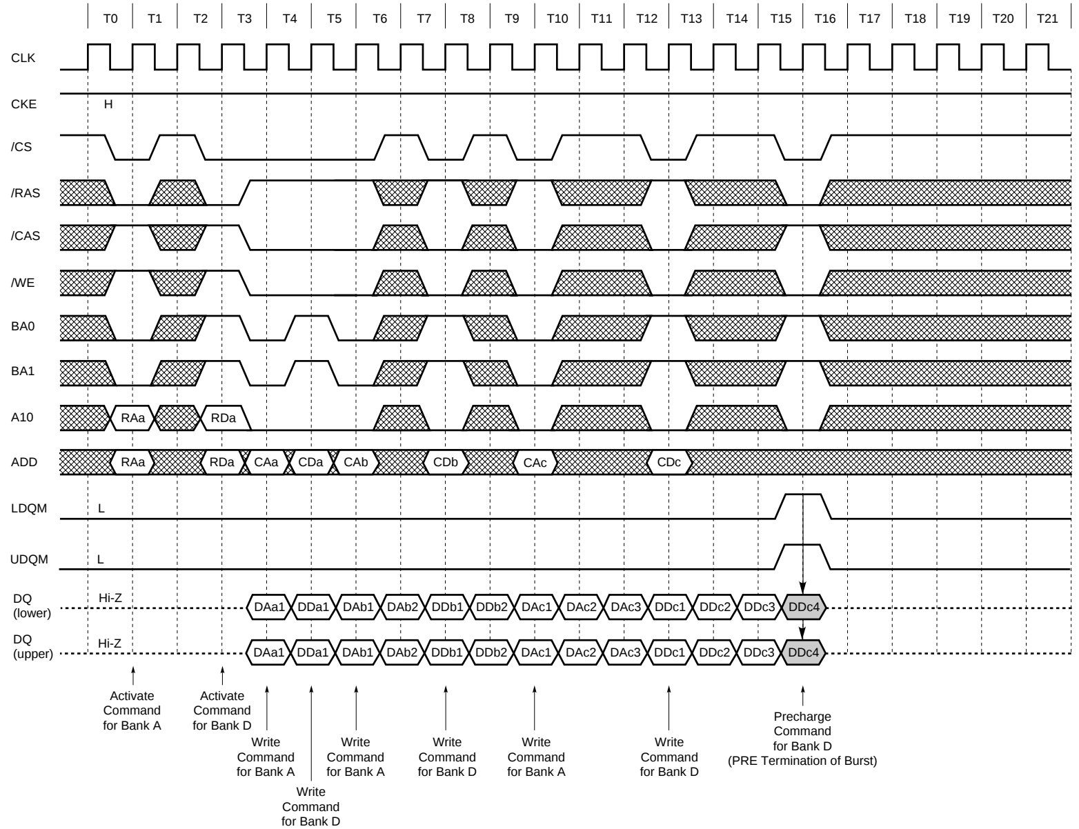
Full Page Random Column Write (Burst Length = Full Page, /CAS Latency = 3)
