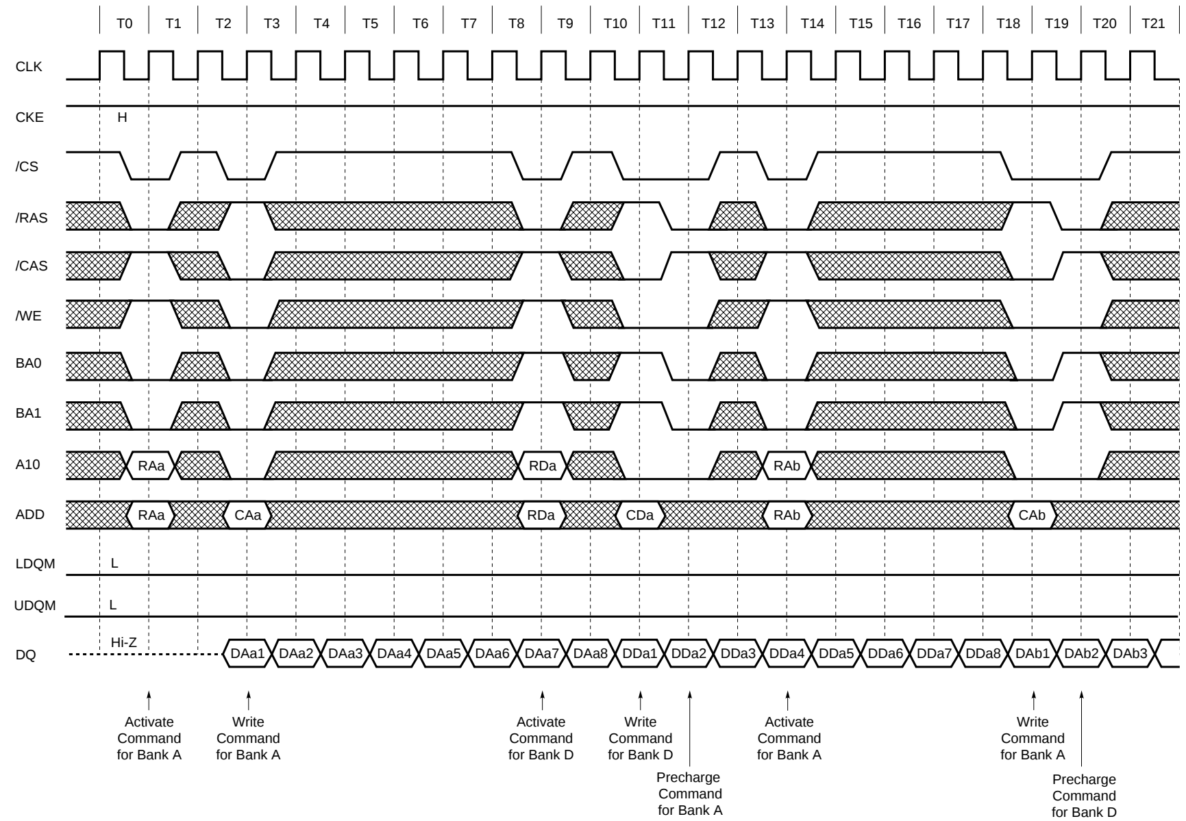
13.15 Random Row Write (Ping-Pong Banks) (1/2) (Burst Length = 8, /CAS Latency = 2)
