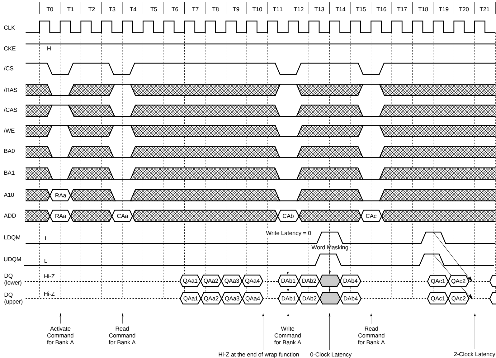
Read and Write (2/2) (Burst Length = 4, /CAS Latency = 3)
