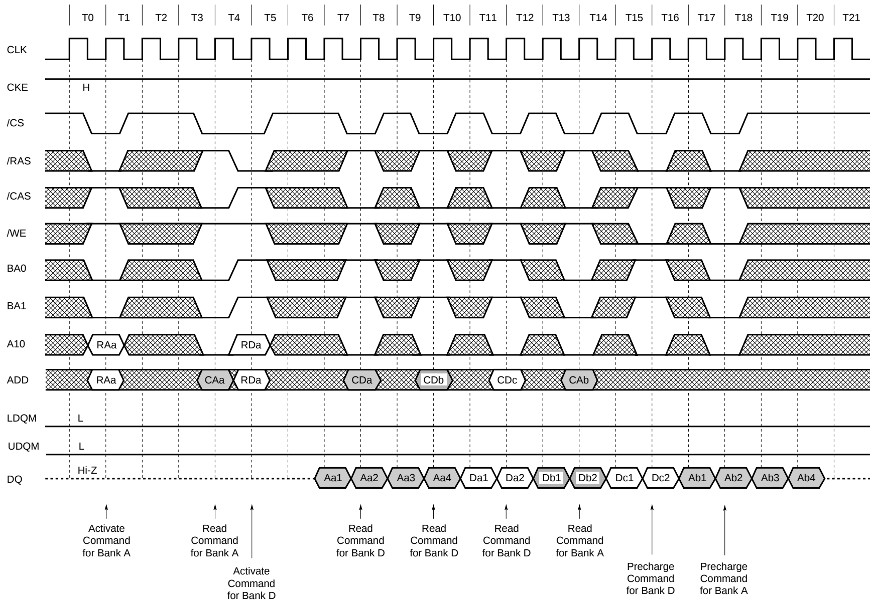
Interleaved Column Read Cycle (2/2) (Burst Length = 4, /CAS Latency = 3)
