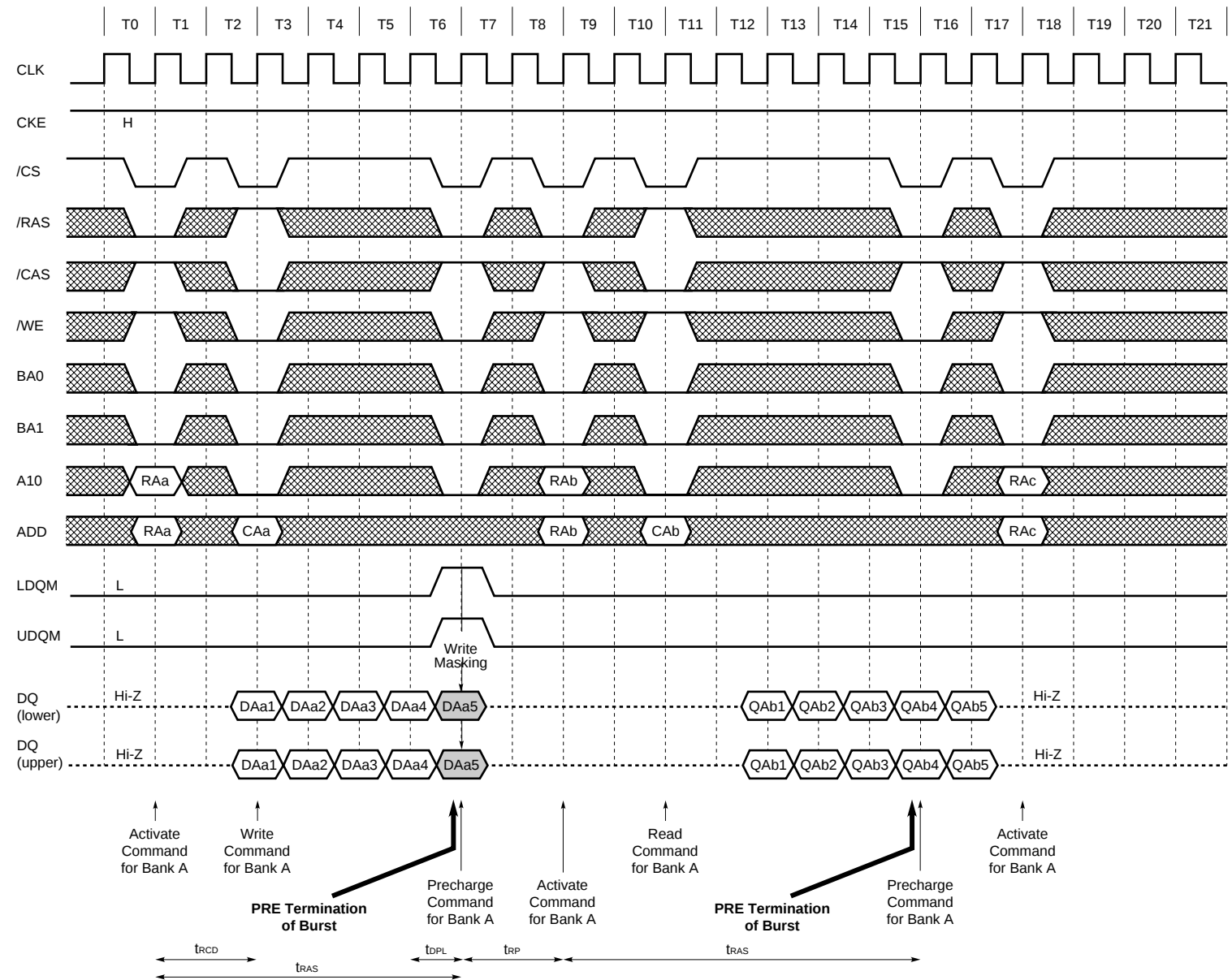
13.27 PRE (Precharge) Termination of Burst (1/2) (Burst Length = 8, /CAS Latency = 2)
