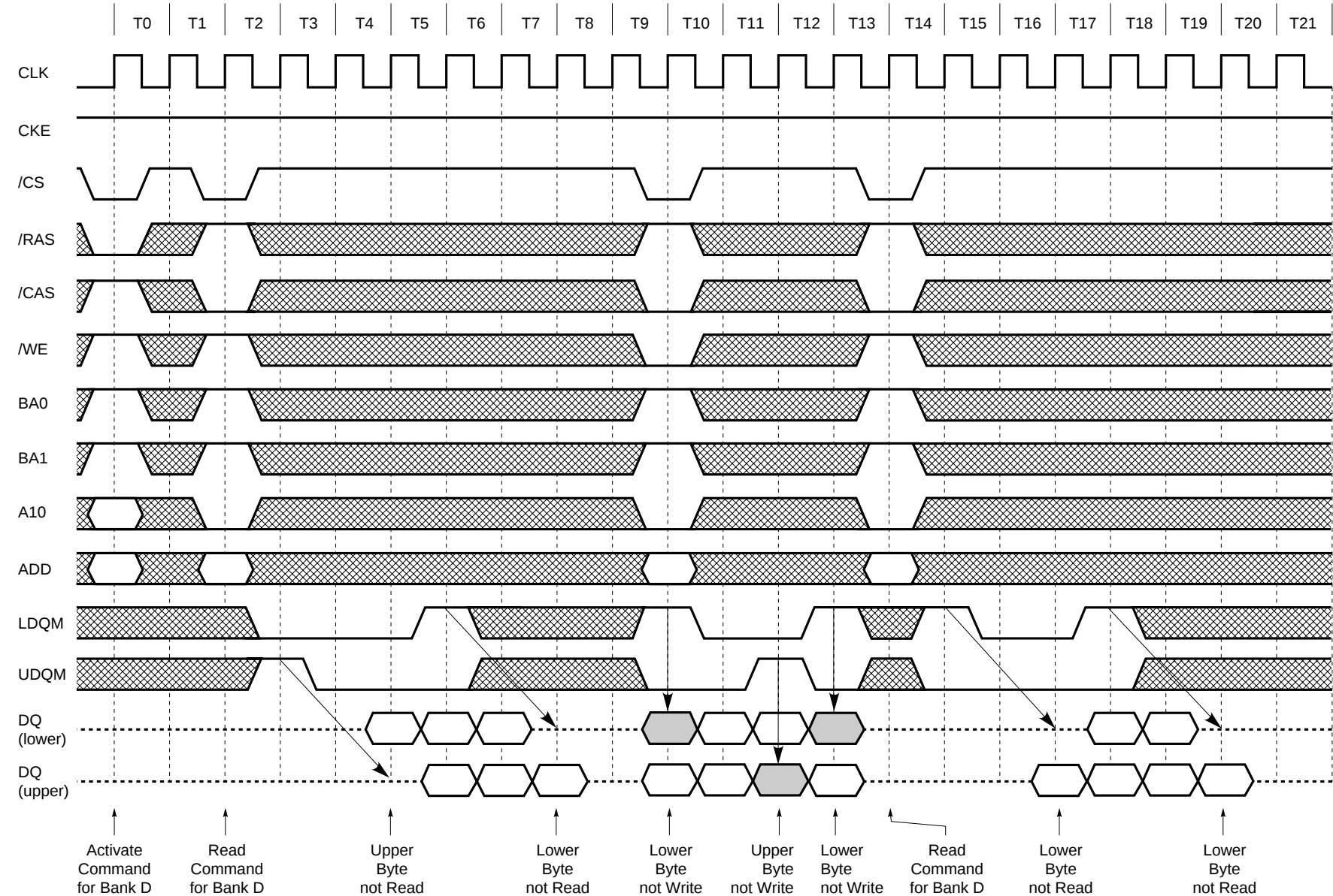
Byte Write Operation (Burst Length = 4, /CAS Latency = 3)
