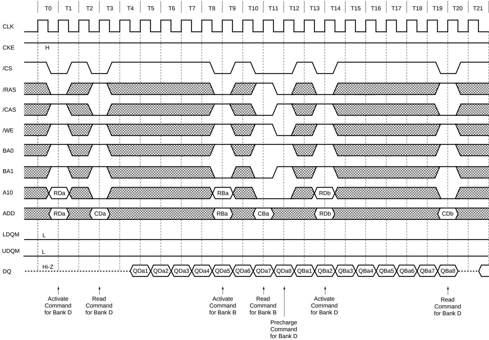
13.14 Random Row Read (Ping-Pong Banks) (1/2) (Burst Length = 8, /CAS Latency = 2)
