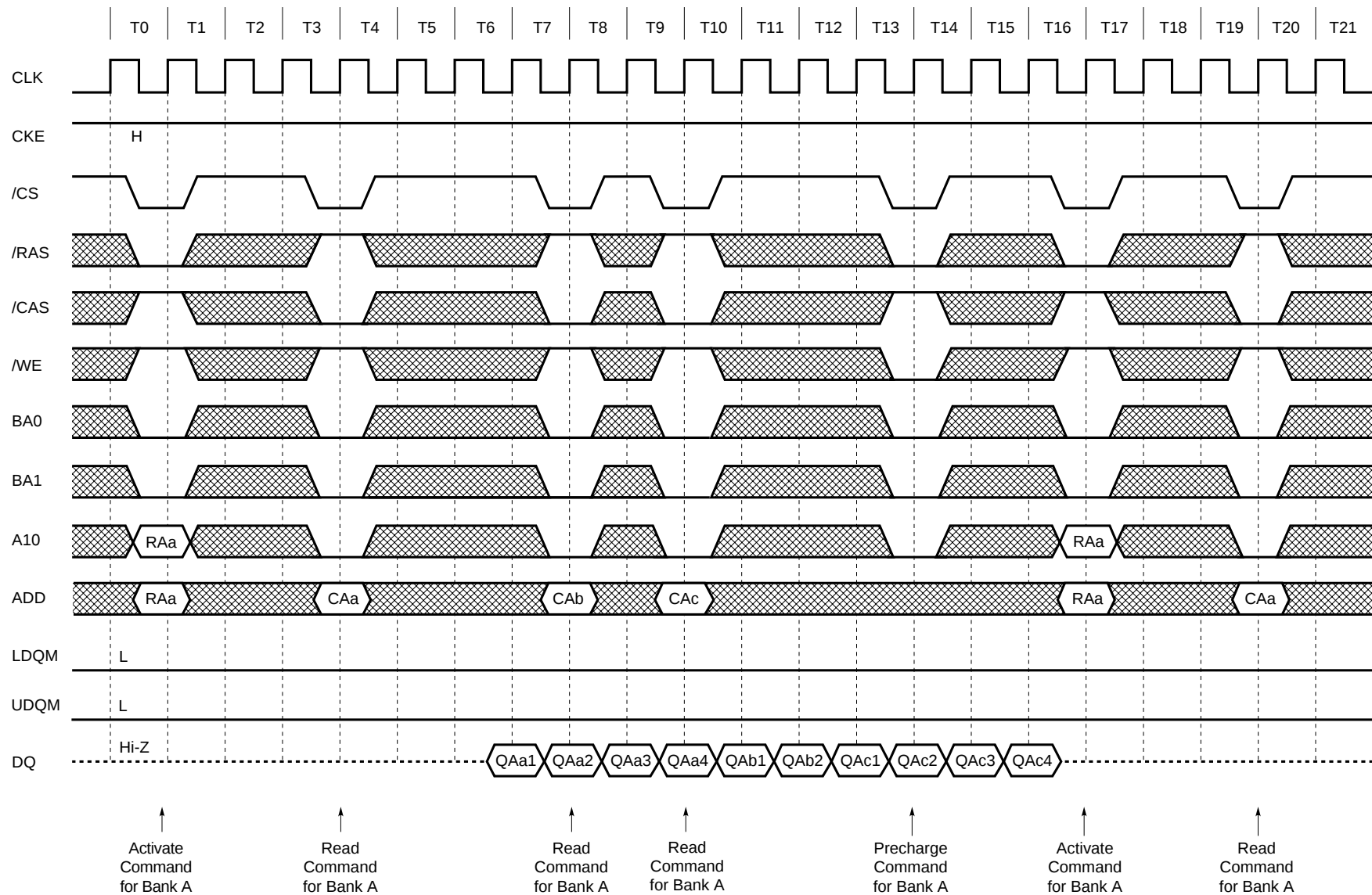
Random Column Read (Page with Same Bank) (2/2) (Burst Length = 4, /CAS Latency = 3)
