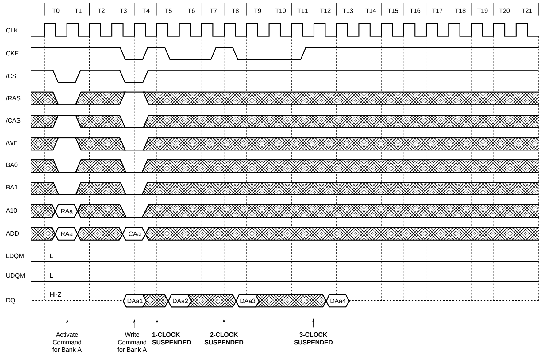
Clock Suspension during Burst Write (using CKE Function) (2/2) (Burst Length = 4, /CAS Latency = 3)
