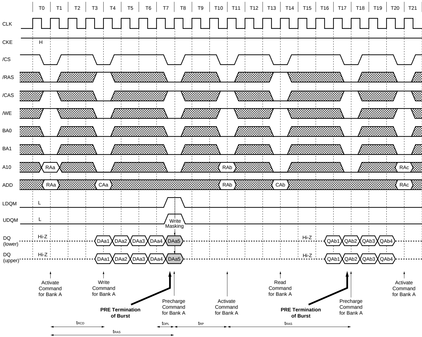
PRE (Precharge) Termination of Burst (2/2) (Burst Length = 8, /CAS Latency = 3)
