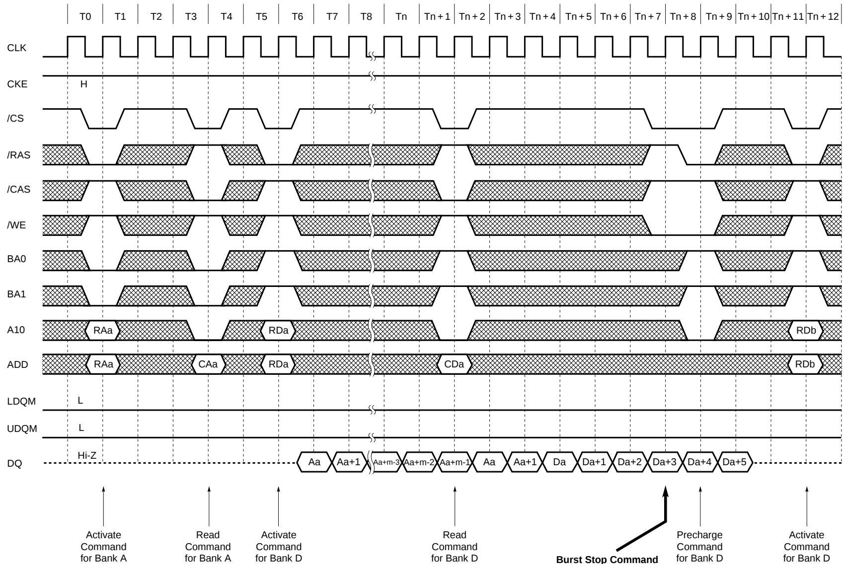
Full Page Read Cycle (2/2) (ICAS latency = 3)
