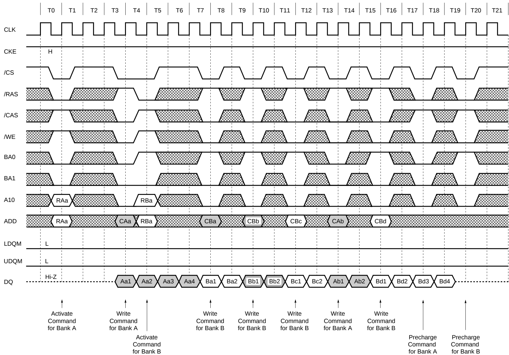
Interleaved Column Write Cycle (2/2) (Burst Length = 4, /CAS Latency = 3)
