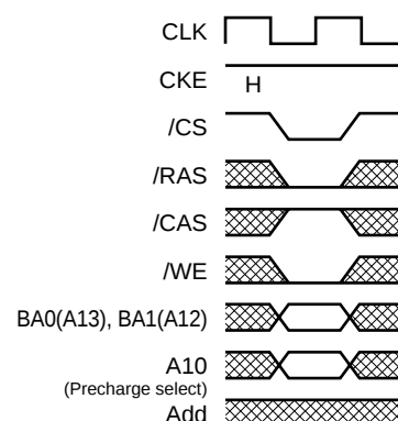
Fig.3 Precharge command
