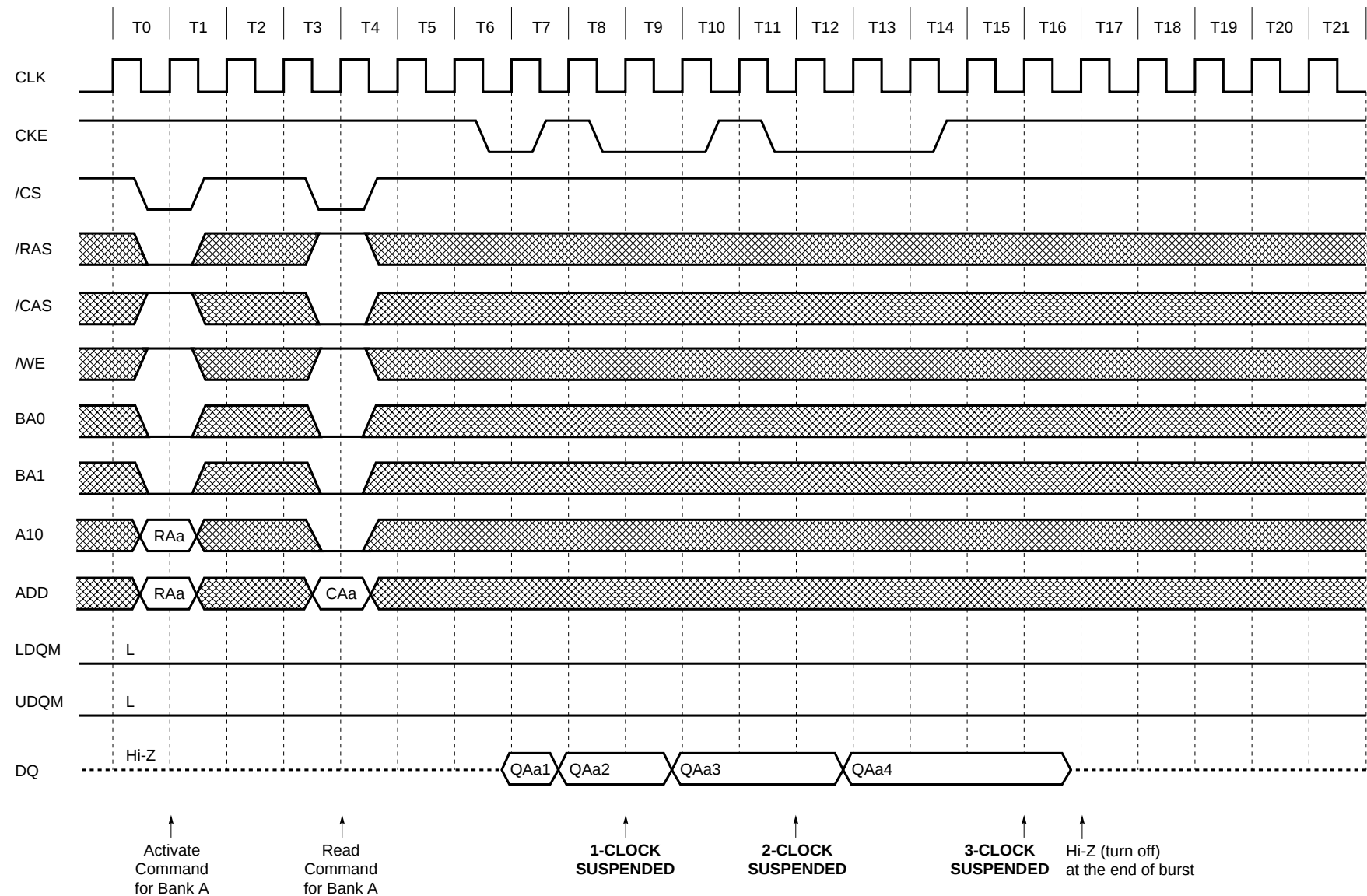
Clock Suspension during Burst Read (using CKE Function) (2/2) (Burst Length = 4, /CAS Latency = 3)
