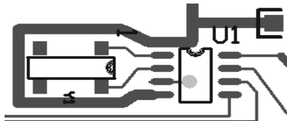
FIGURE 21. SUGGESTED LAYOUT FOR ISL1208 AND CRYSTAL
