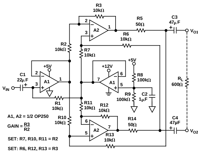
Figure 36. A Low Noise, Single Supply Differential Line Driver
