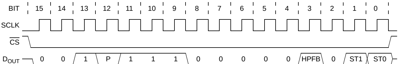
Figure 4-10 Register Write Command Response
