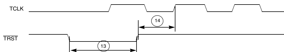
Figure 14. TRST Timing
