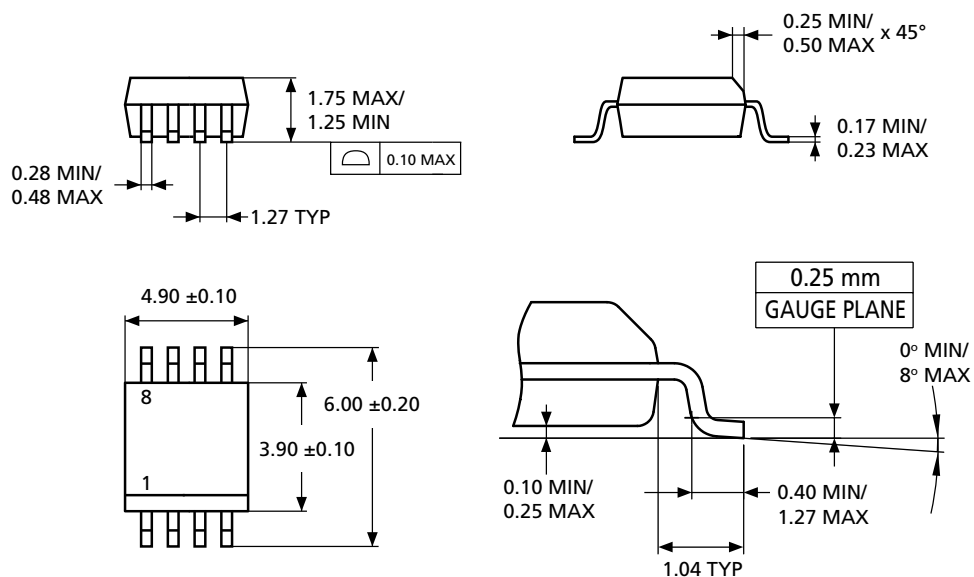
Figure 31: SO8N – 8 lead plastic small outline, 150 mils body width
