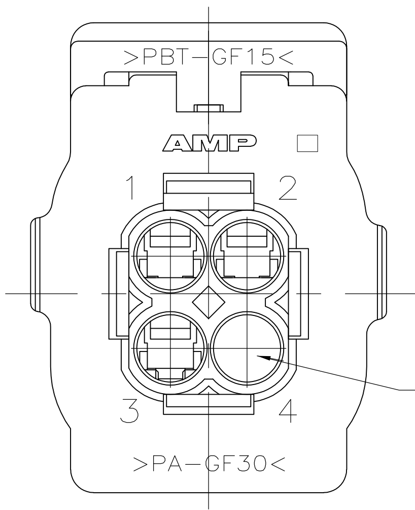
VIEW B-B
