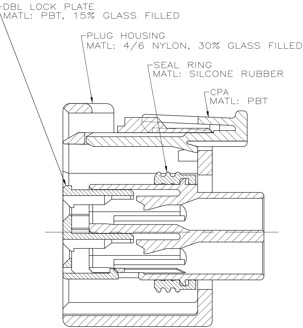
SECTION Z-Z
