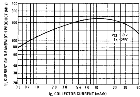
FIGURE 6 - CURRENT-GAIN-BANDWIDTH PRODUCT
