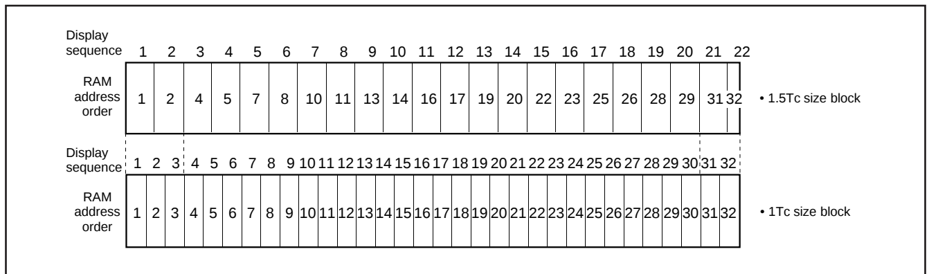
Fig. 12.11.22 RAM Data for 3rd Character
