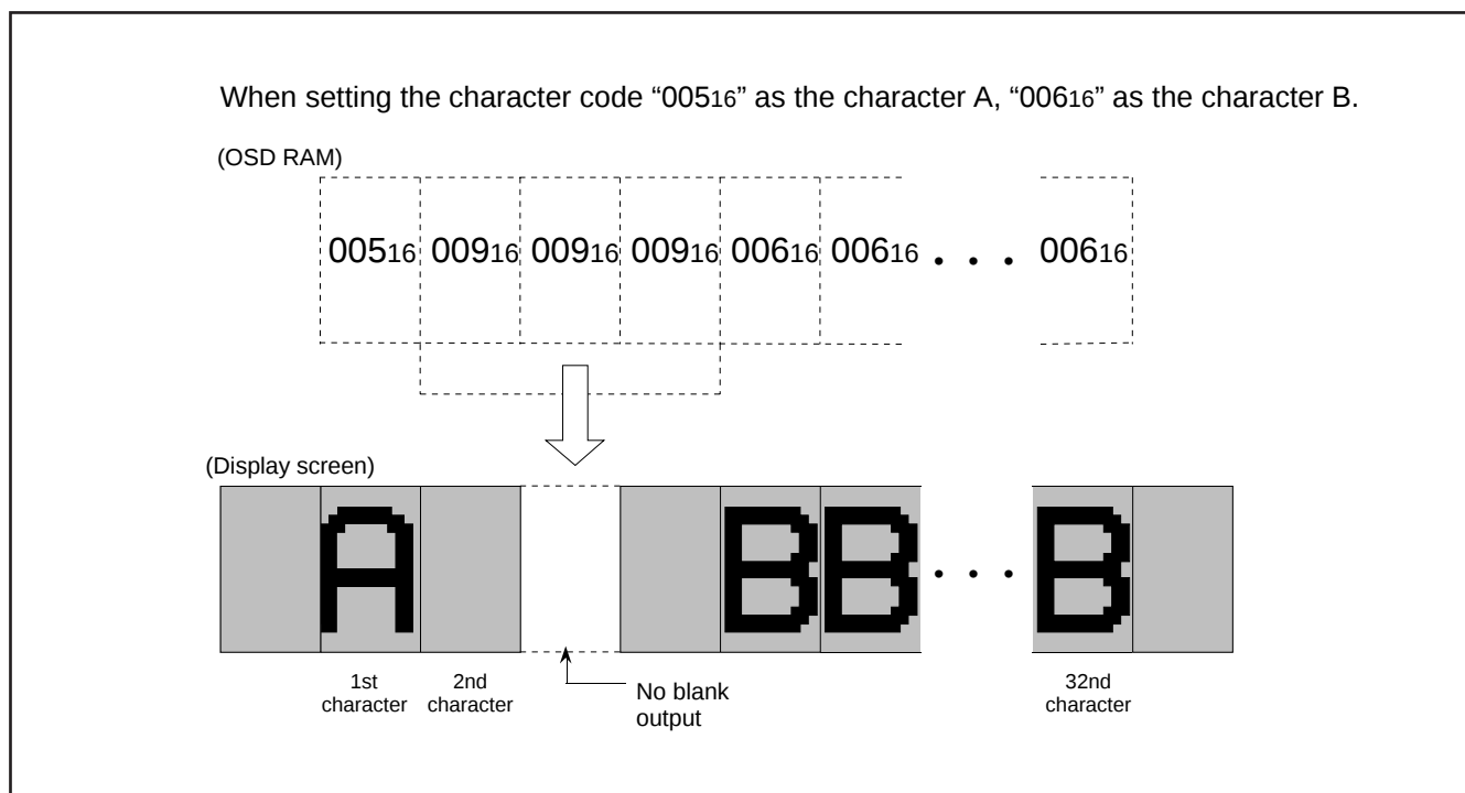
Fig. 12.11.37 Display Screen Example of Automatic Solid Space
