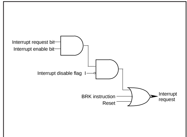
Fig. 12.3.1 Interrupt Control
