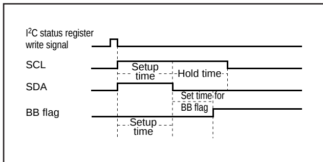
Fig. 12.6.9 START Condition Generation Timing Diagram
