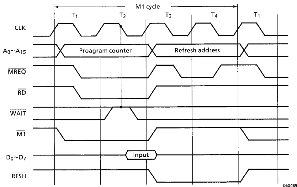
Figure 3.11 Opcode Fetch Timing
