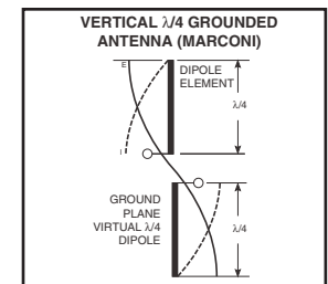
Figure 23: Dipole Antenna
