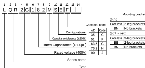
Type numbering system (Example : 400V 1800μF)
