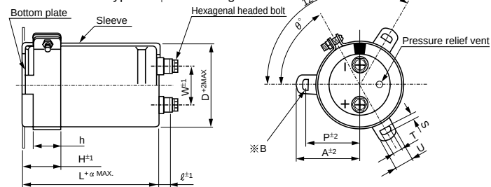
Screw terminal type for φ51 and larger
