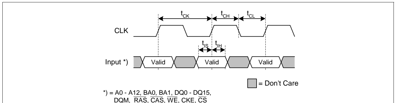
Figure 8 Address / Command Inputs Timing Parameters
