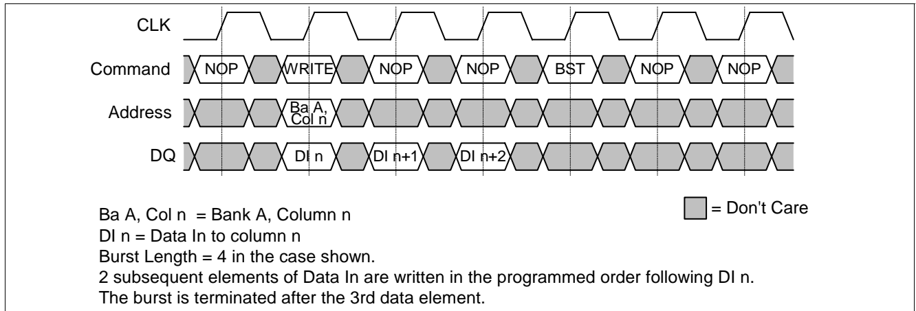
Figure 33 Terminating a WRITE Burst
