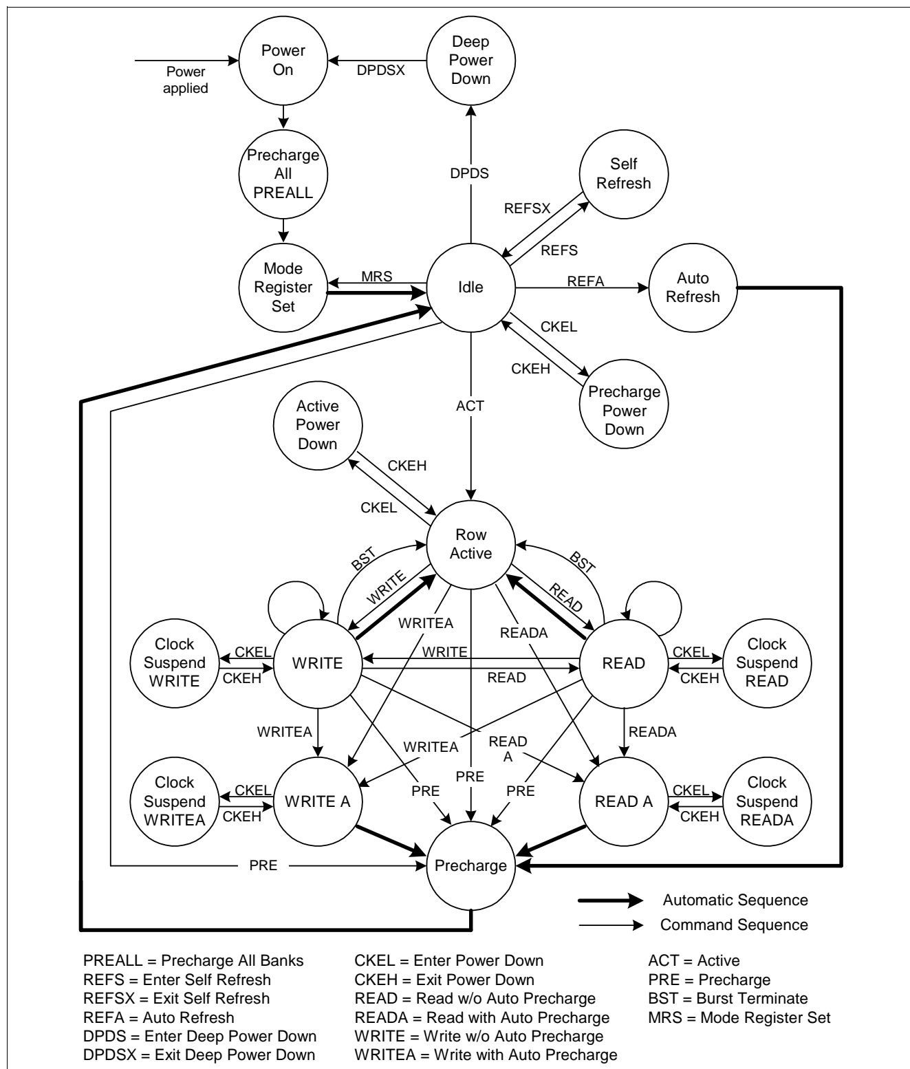
Figure 7 State Diagram
