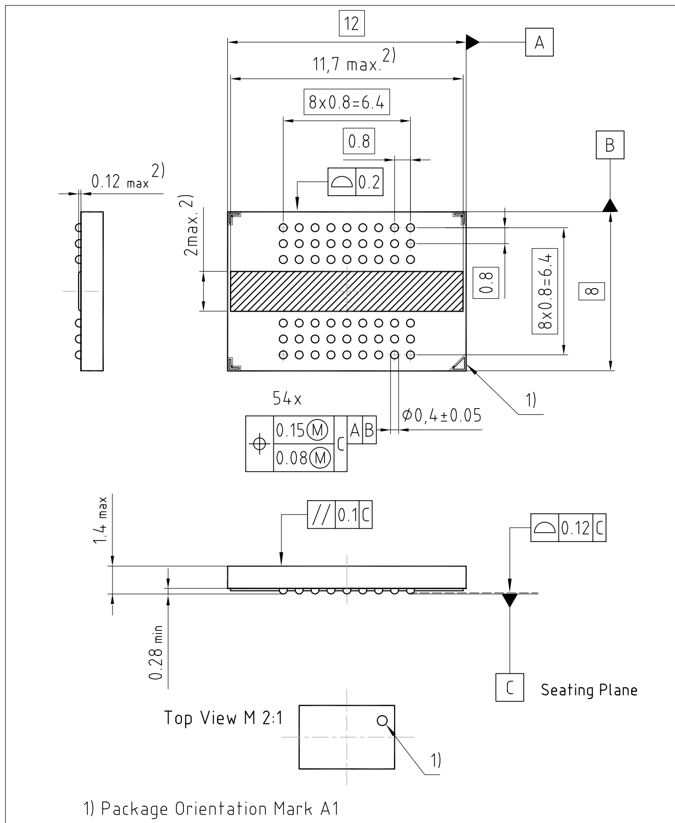
Figure 50 Package FBGA-54
