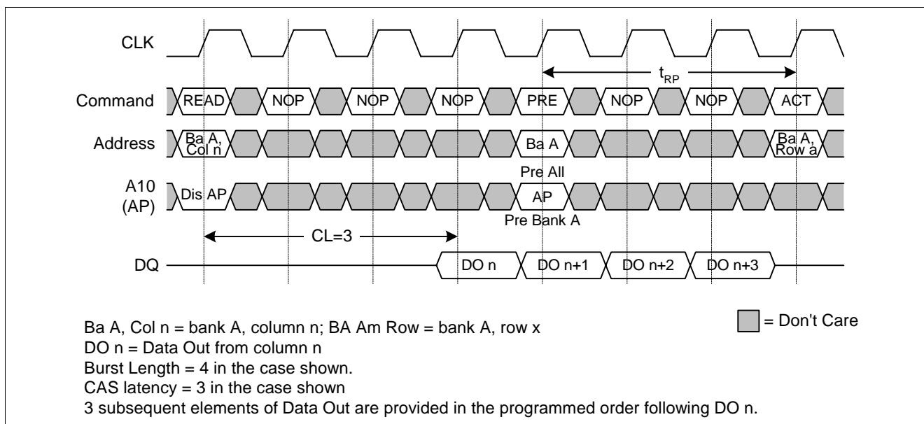
Figure 25 READ to PRECHARGE Timing
