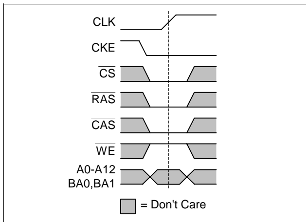
Figure 46 SELF REFRESH Entry Command
