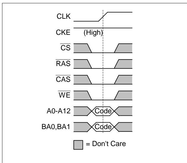
Figure 10 Mode Register Set Command
