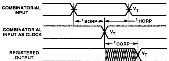
Output Register (PT Clock)
