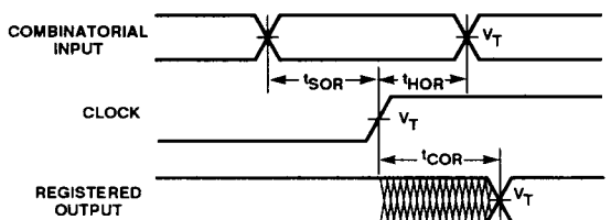
Output Register (Pin Clock)
