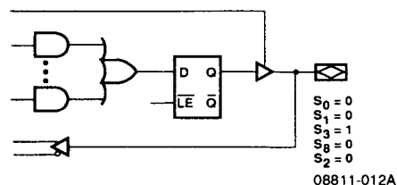
Figure 3b. Single Feedback Macrocells
