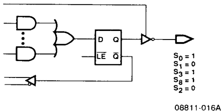
Figure 3b. Single Feedback Macrocells (Continued)
