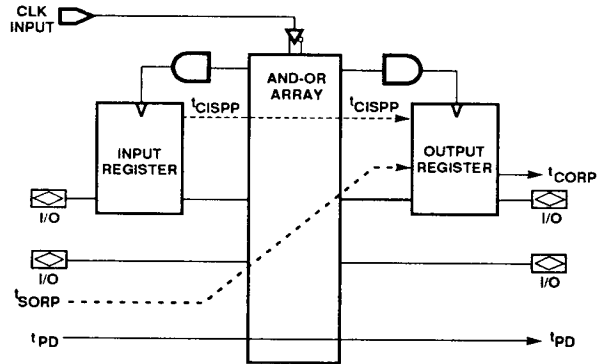
Input/Output Register Specs (PT CLK Reference)
