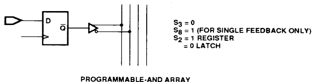
Figure 3c. All Macrocells
