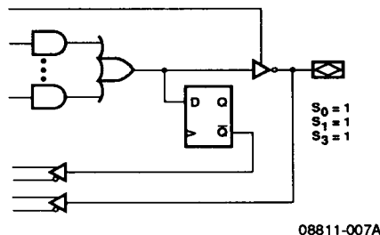
Output Combinatorial/Active High
