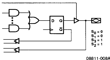
Figure 3a. Dual Feedback Macrocells
