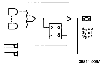
Figure 3a. Dual Feedback Macrocells
