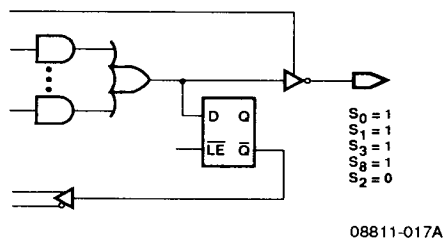
Figure 3b. Single Feedback Macrocells (Continued)
