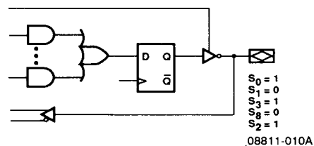
Output Registered/Active Low, I/O Feedback
