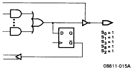
Output Combinatorial/Active Low, Latched Feedback
