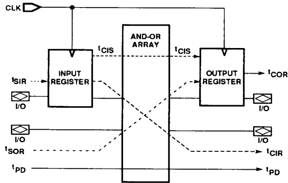
Input/Output Register Specs (Pin CLK Reference)
