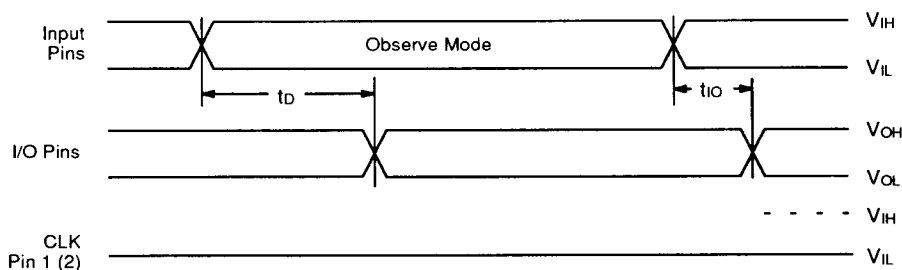
Observability Waveform
