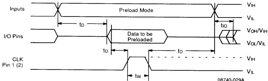
Preload Waveform
