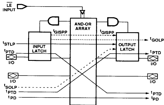
Input/Output Latch Specs (PT \overline{LE} Reference)
