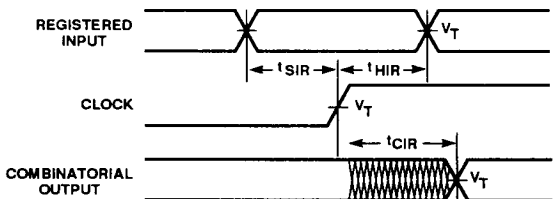
Input Register
