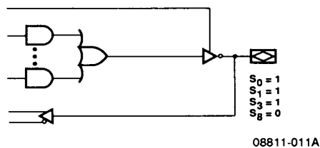
Output Combinatorial/Active Low, I/O Feedback
