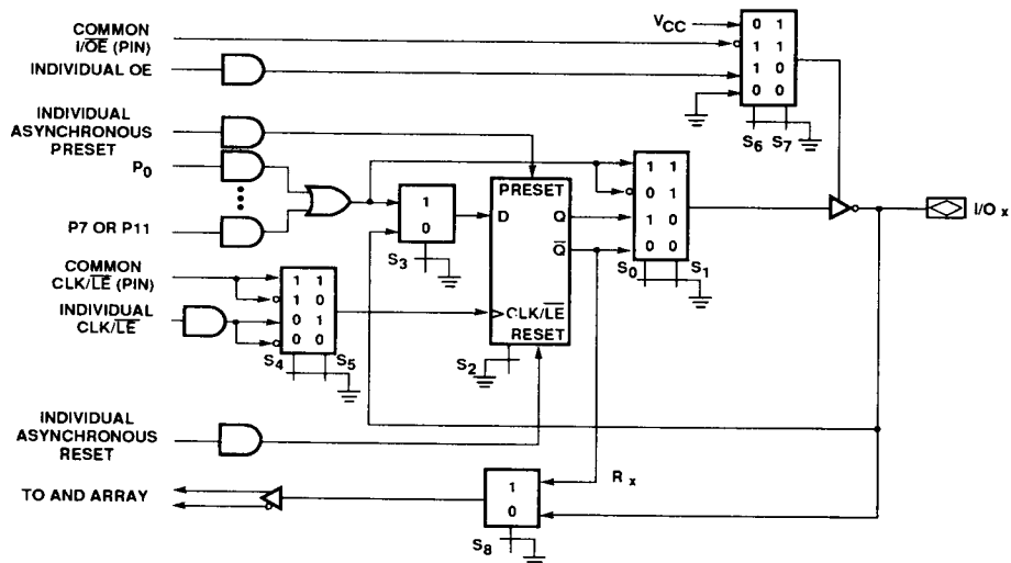
Figure 2a. PALCE29MA16 Macrocell (Single Feedback)
