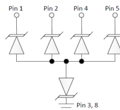
Schematic Diagram
