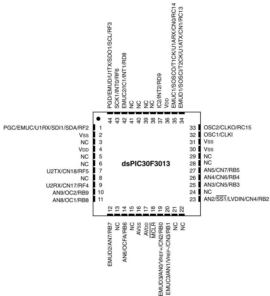
44-Pin QFN
