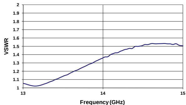
VSWR (13-15 GHz)
