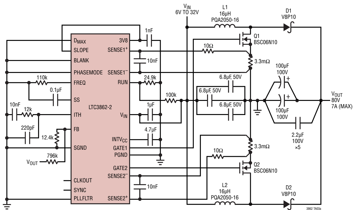
A 6V to 32V Input, 80V/7A Output 2-Phase Boost Converter Application Circuit
